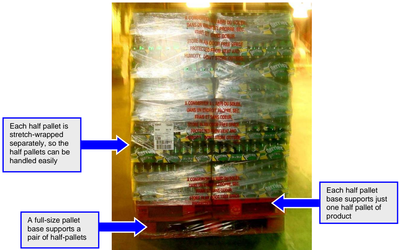
Figure 5-2 Example of half-pallet GTIN 03179730107765
